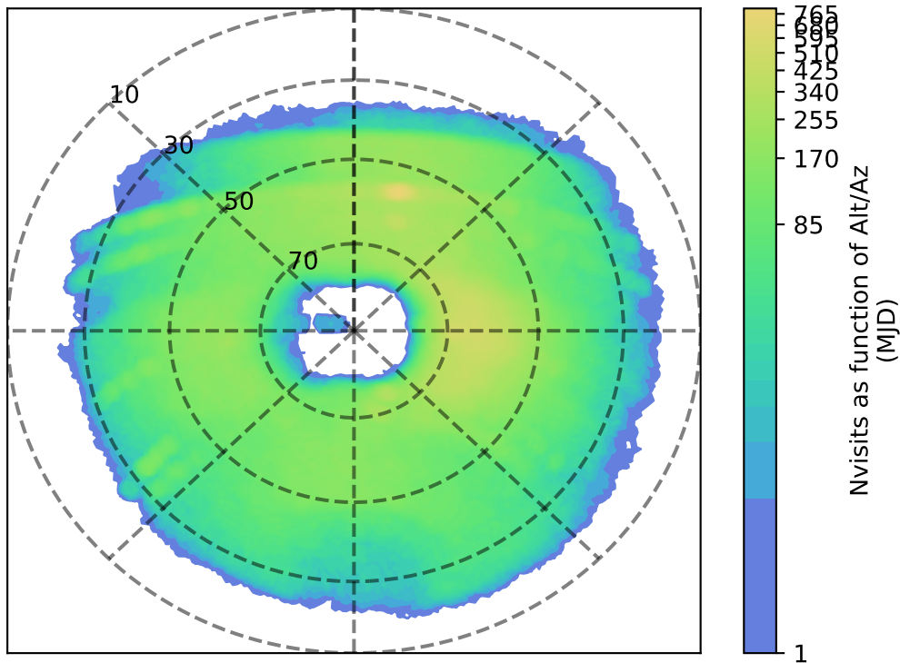
weather_cloudso12v3.4_10yrs u: Nvisits as function of Alt/Az
