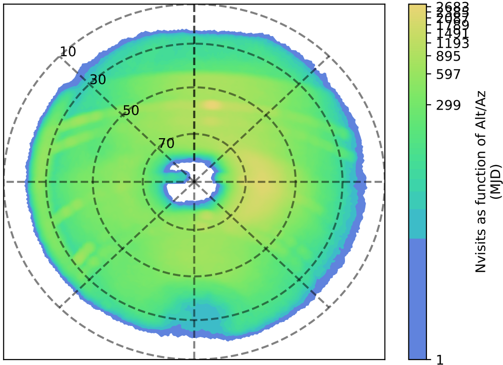
weather_cloudso12v3.4_10yrs r: Nvisits as function of Alt/Az
