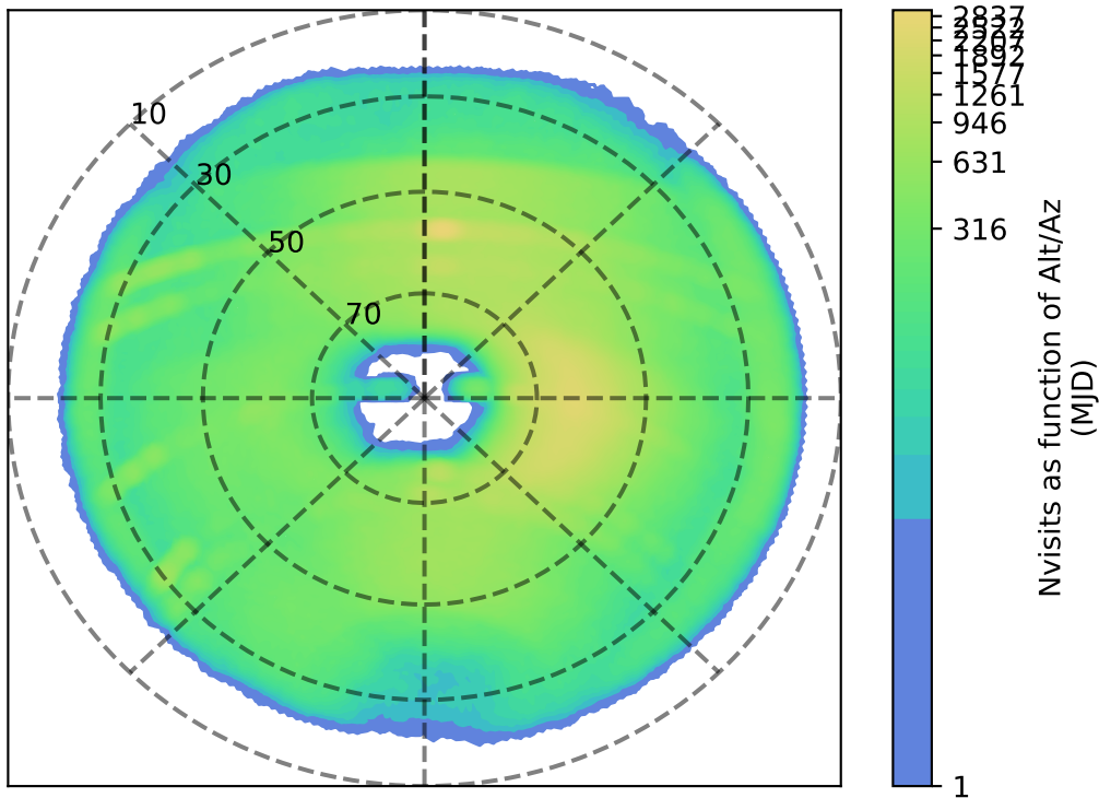
weather_cloudso12v3.4_10yrs i: Nvisits as function of Alt/Az
