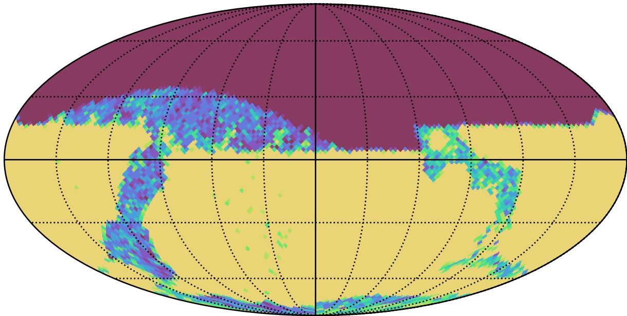
weather_cloudso12v3.4_10yrs z and night < 365: N year 1
