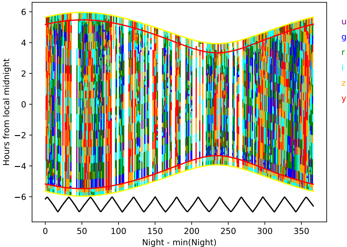
weather_cloudso12v3.4_10yrs year 9-10: Hourglass
