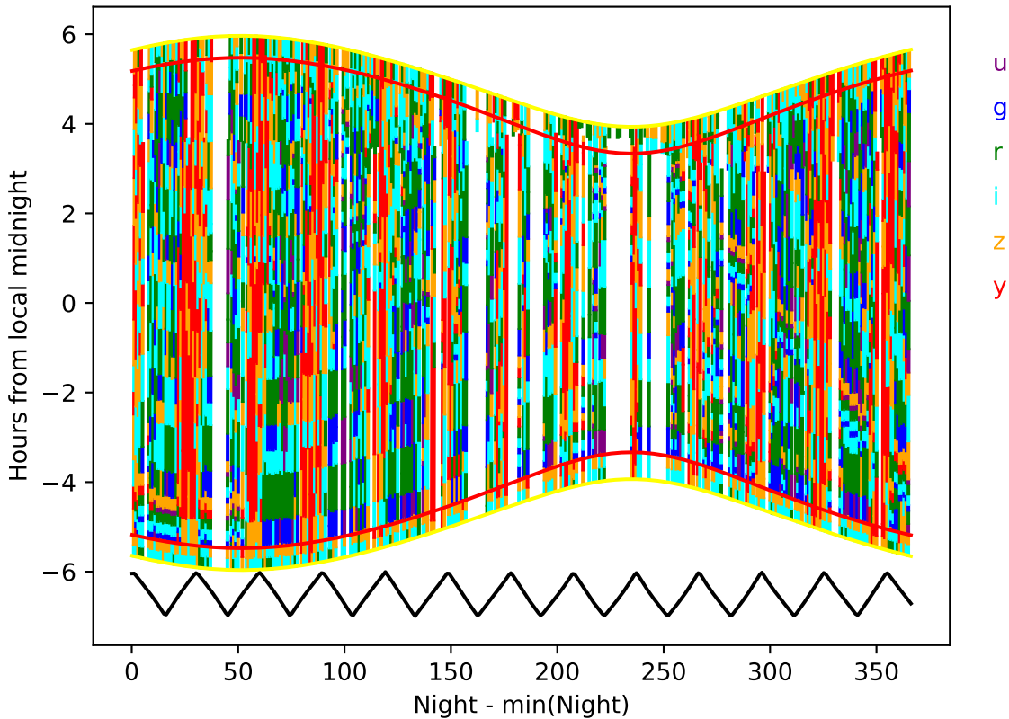
weather_cloudso12v3.4_10yrs year 1-2: Hourglass
