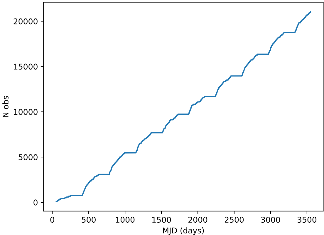
weather_cloudso12v3.4_10yrs note like DD:ELAISS1%: Cumulative
