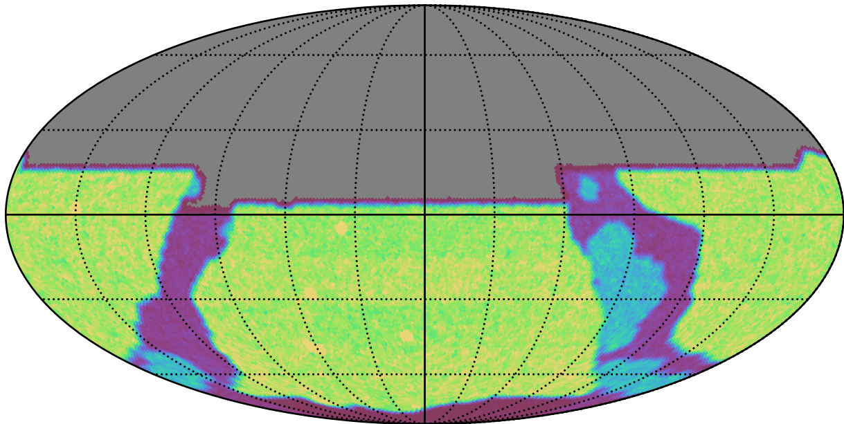
weather_cloudso12v3.4_10yrs y: Count observationStartMJD
