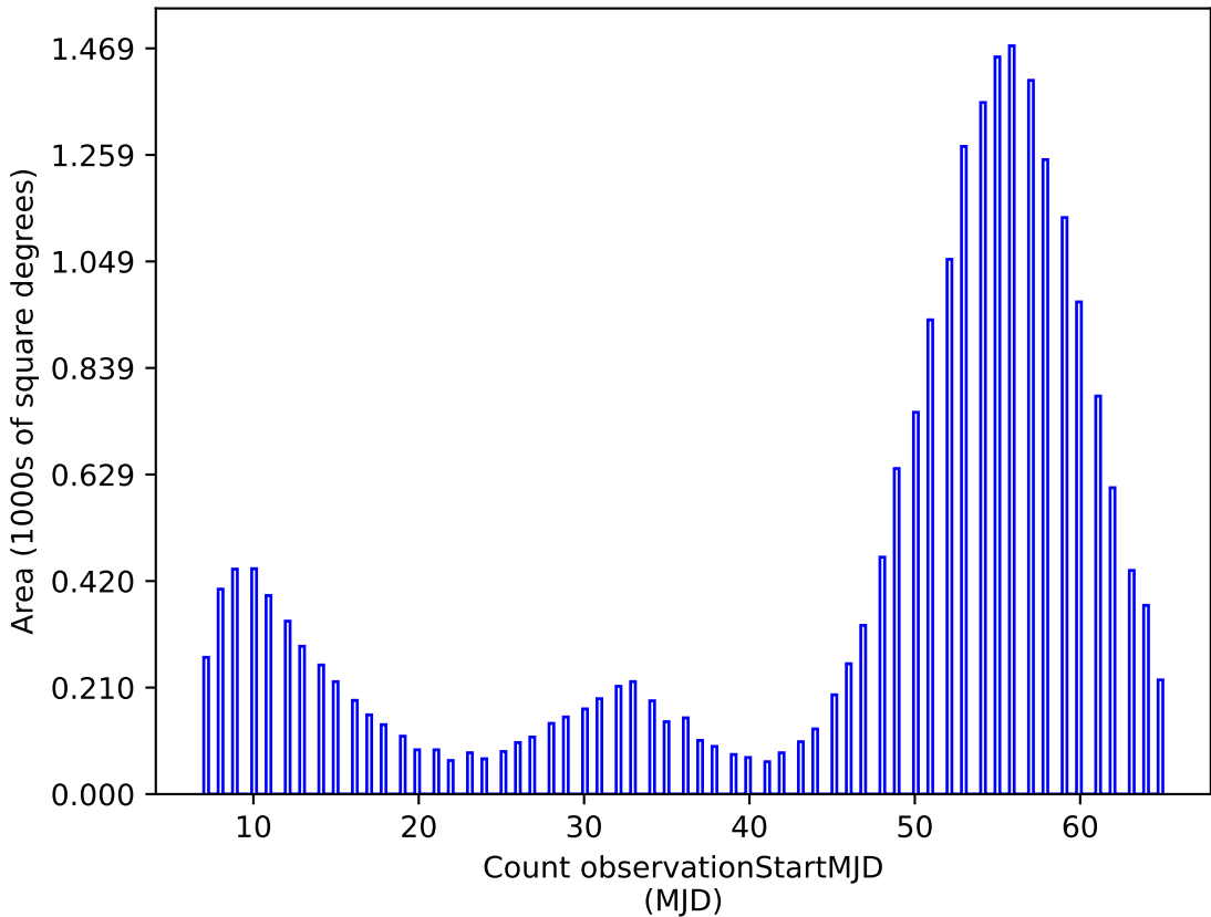
weather_cloudso12v3.4_10yrs u: Count observationStartMJD
