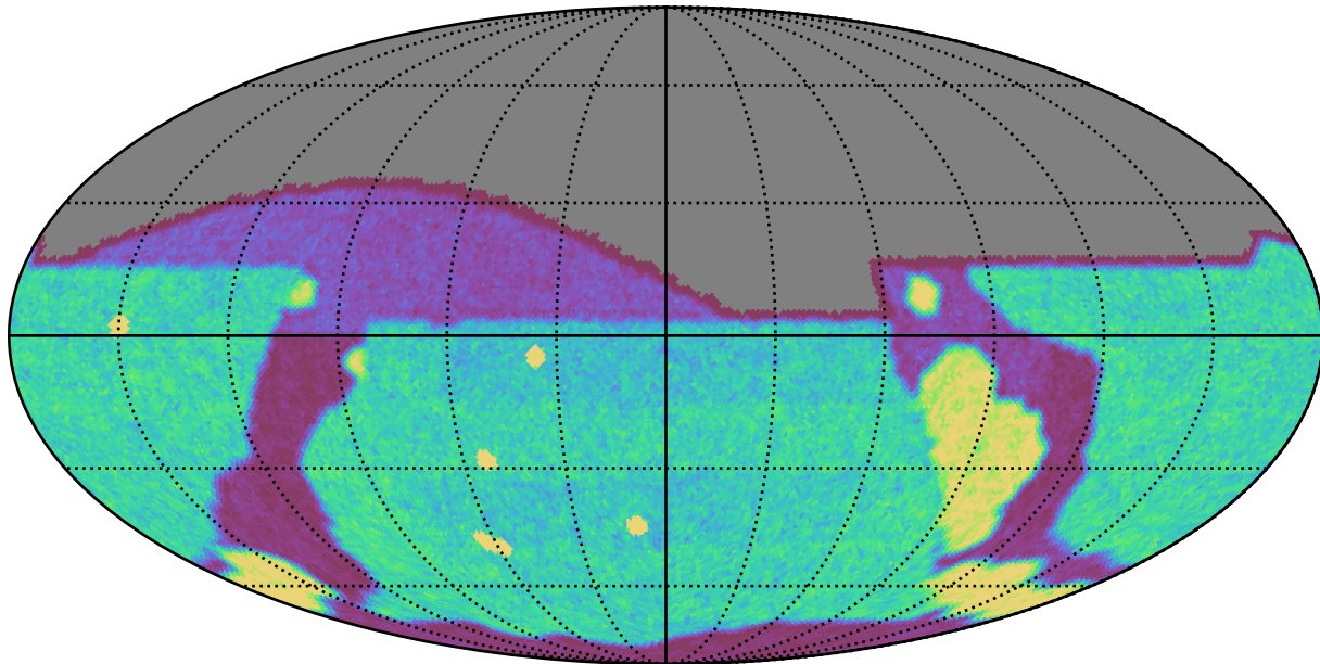
weather_cloudso12v3.4_10yrs g: Count observationStartMJD
