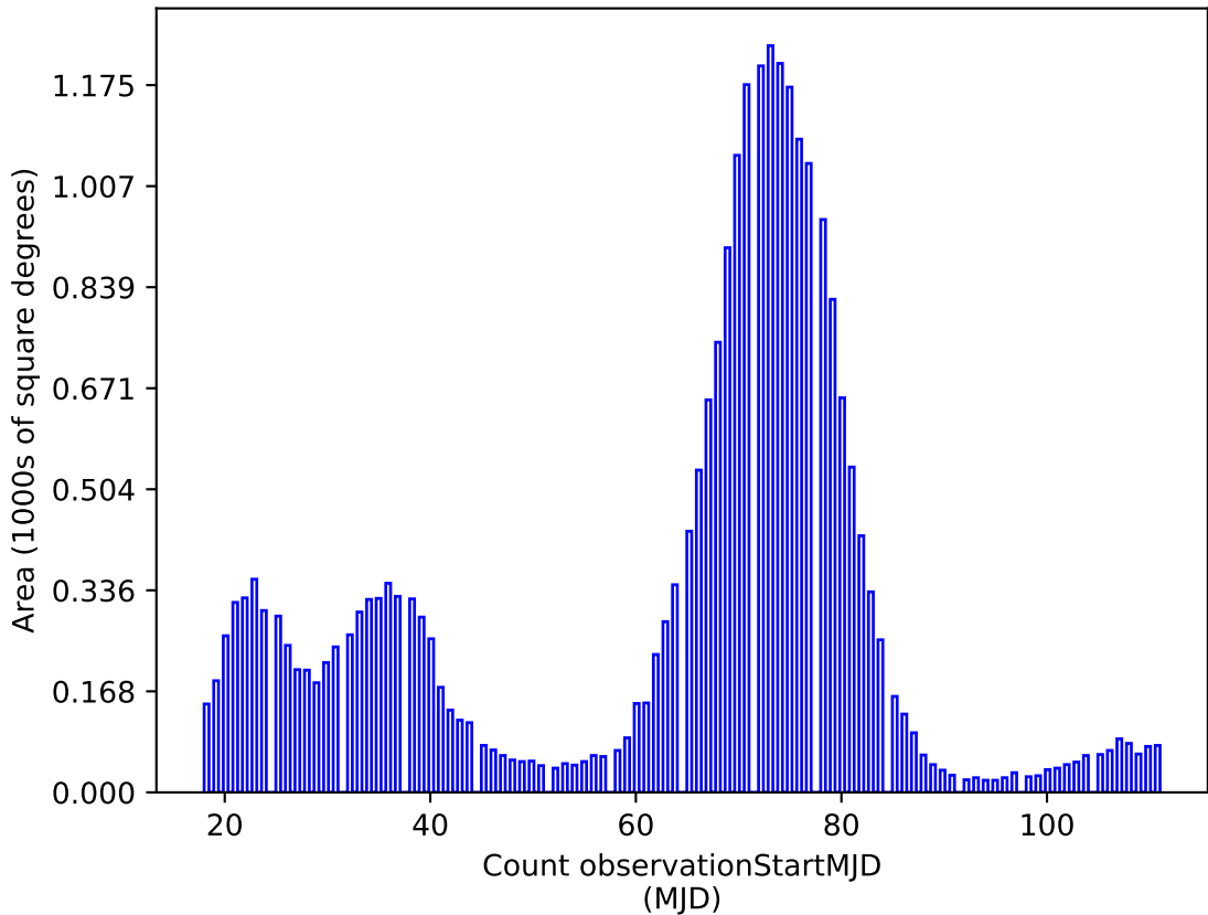
weather_cloudso12v3.4_10yrs g: Count observationStartMJD
