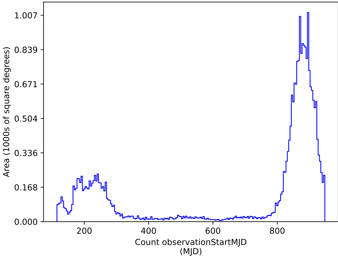
weather_cloudso12v3.4_10yrs : Count observationStartMJD
