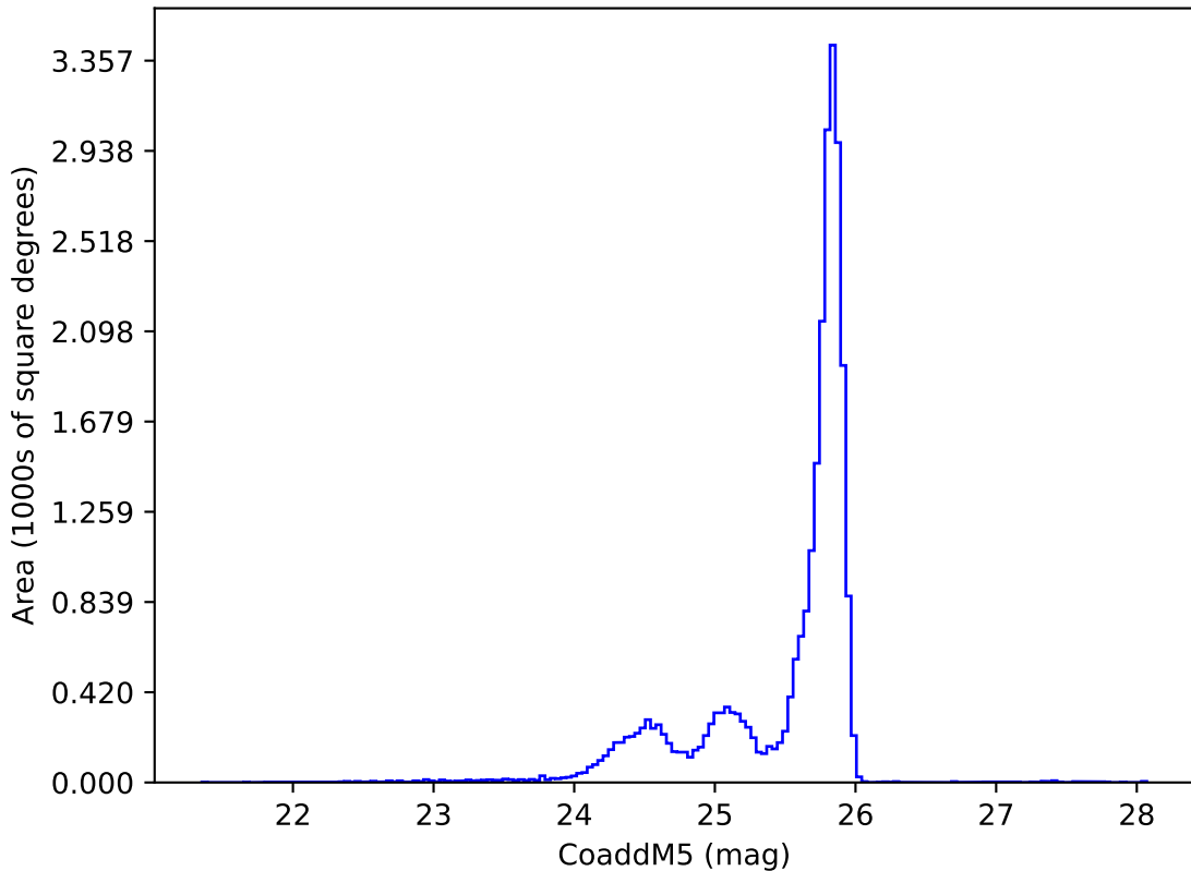
weather_cloudso12v3.4_10yrs z: CoaddM5
