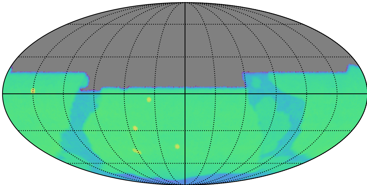
weather_cloudso12v3.4_10yrs y: CoaddM5
