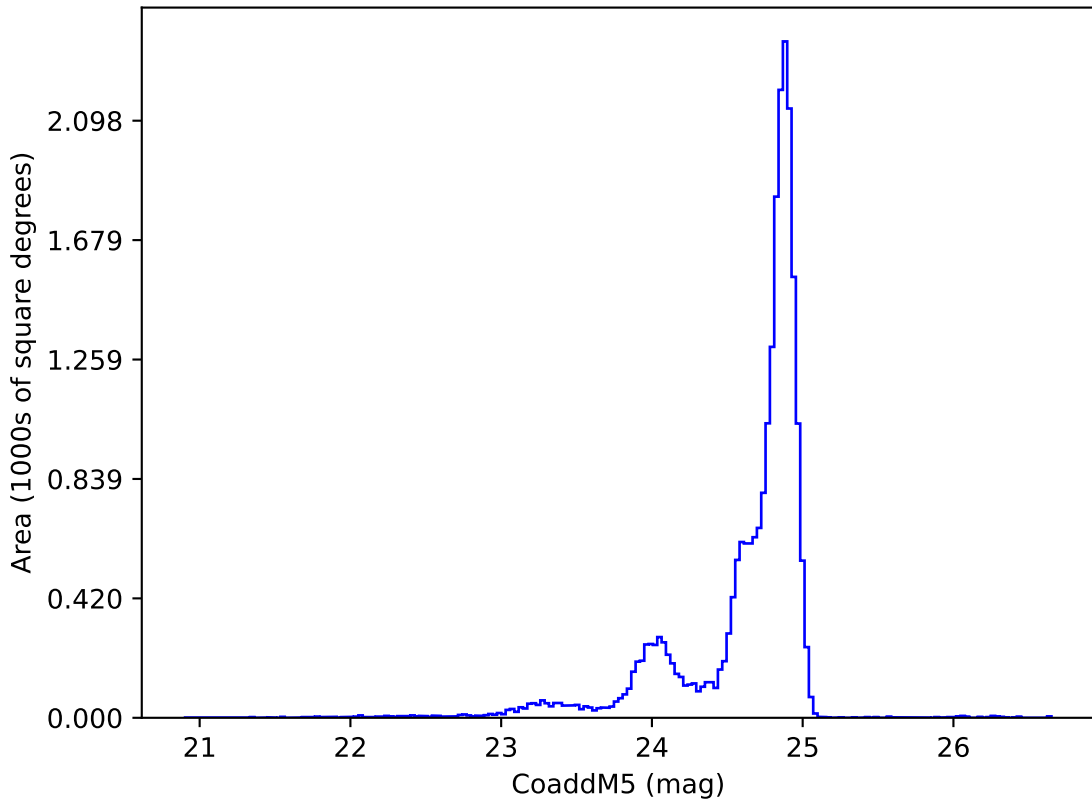
weather_cloudso12v3.4_10yrs y: CoaddM5
