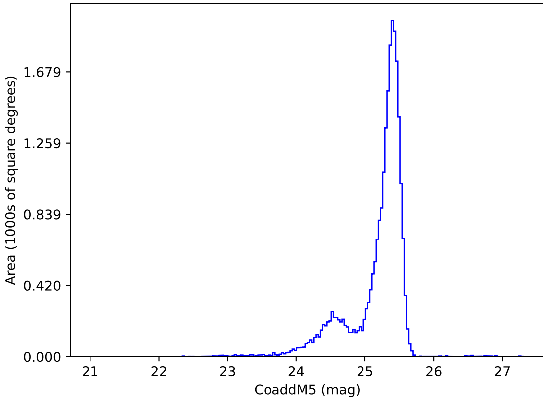
weather_cloudso12v3.4_10yrs u: CoaddM5
