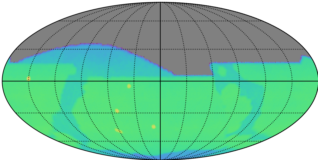
weather_cloudso12v3.4_10yrs r: CoaddM5
