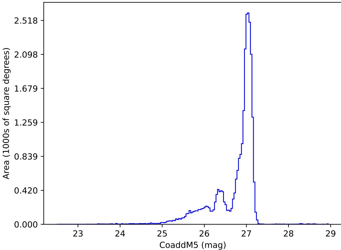
weather_cloudso12v3.4_10yrs r: CoaddM5
