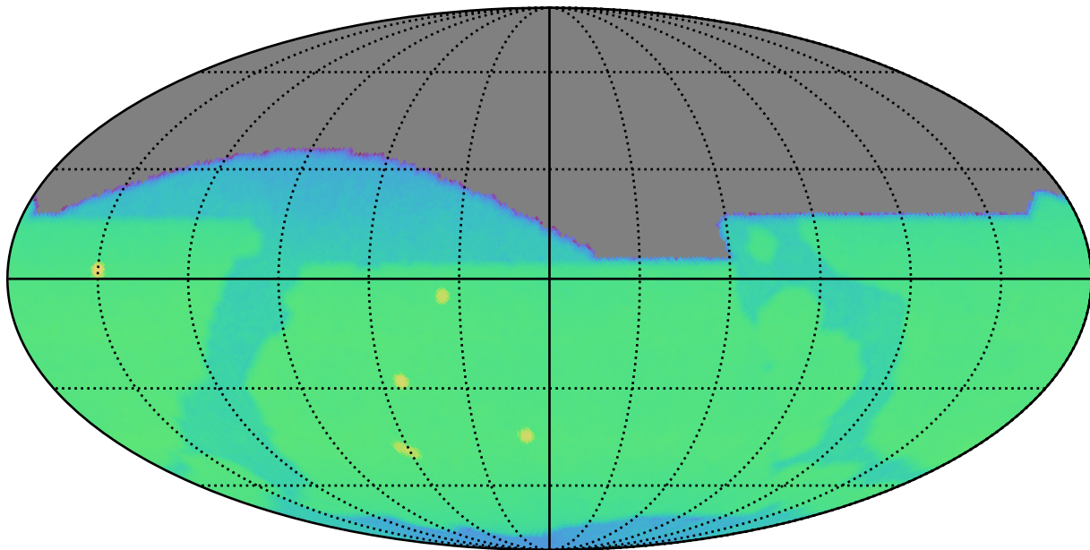
weather_cloudso12v3.4_10yrs i: CoaddM5
