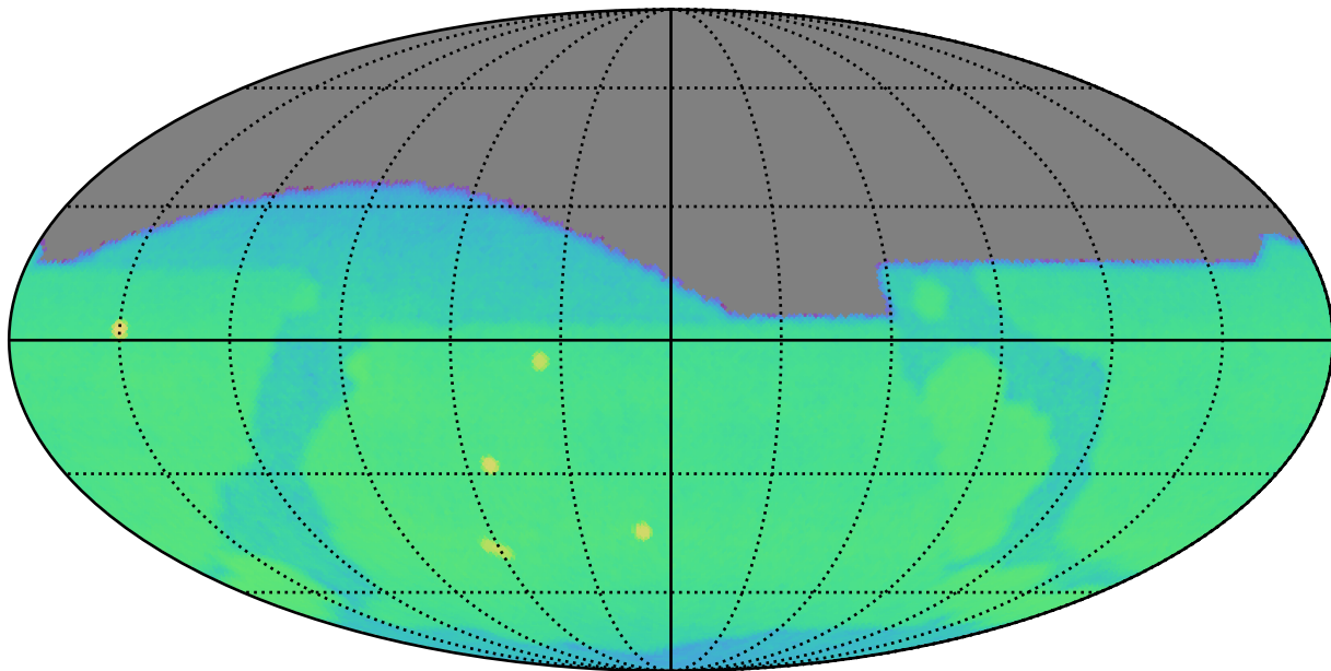
weather_cloudso12v3.4_10yrs g: CoaddM5
