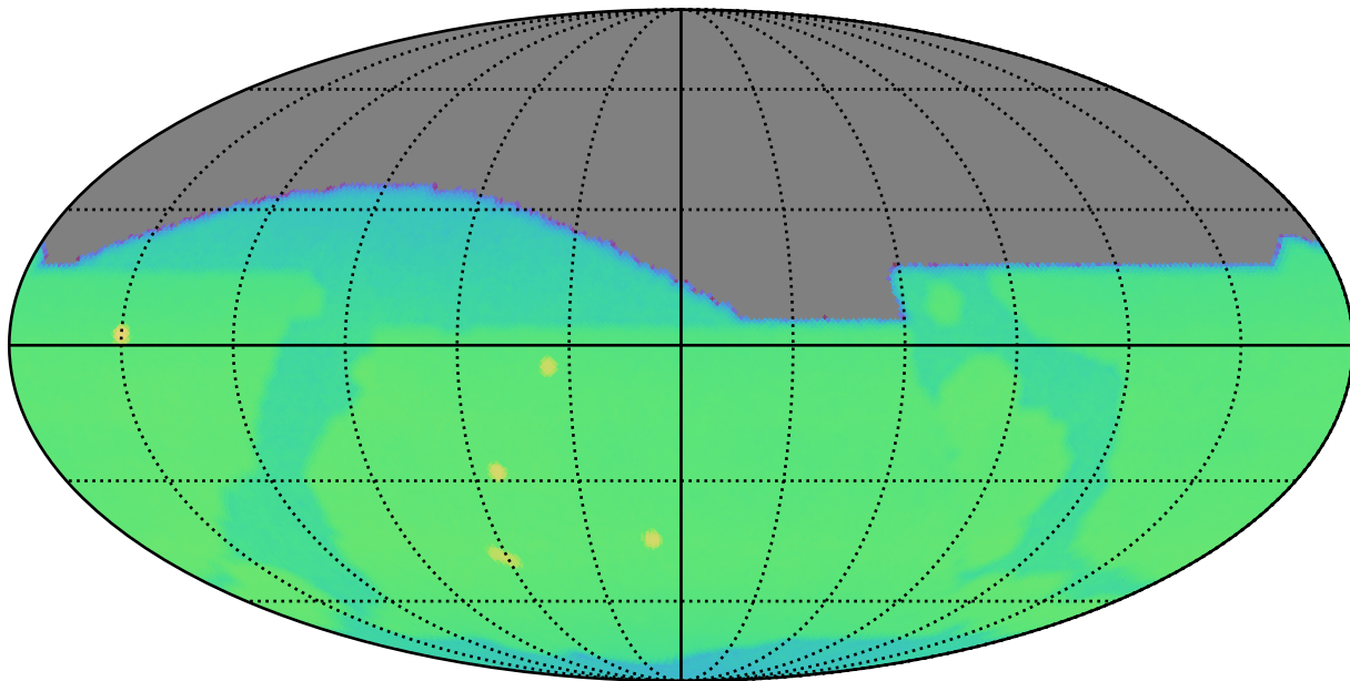
weather_cloudso12v3.4_10yrs : CoaddM5
