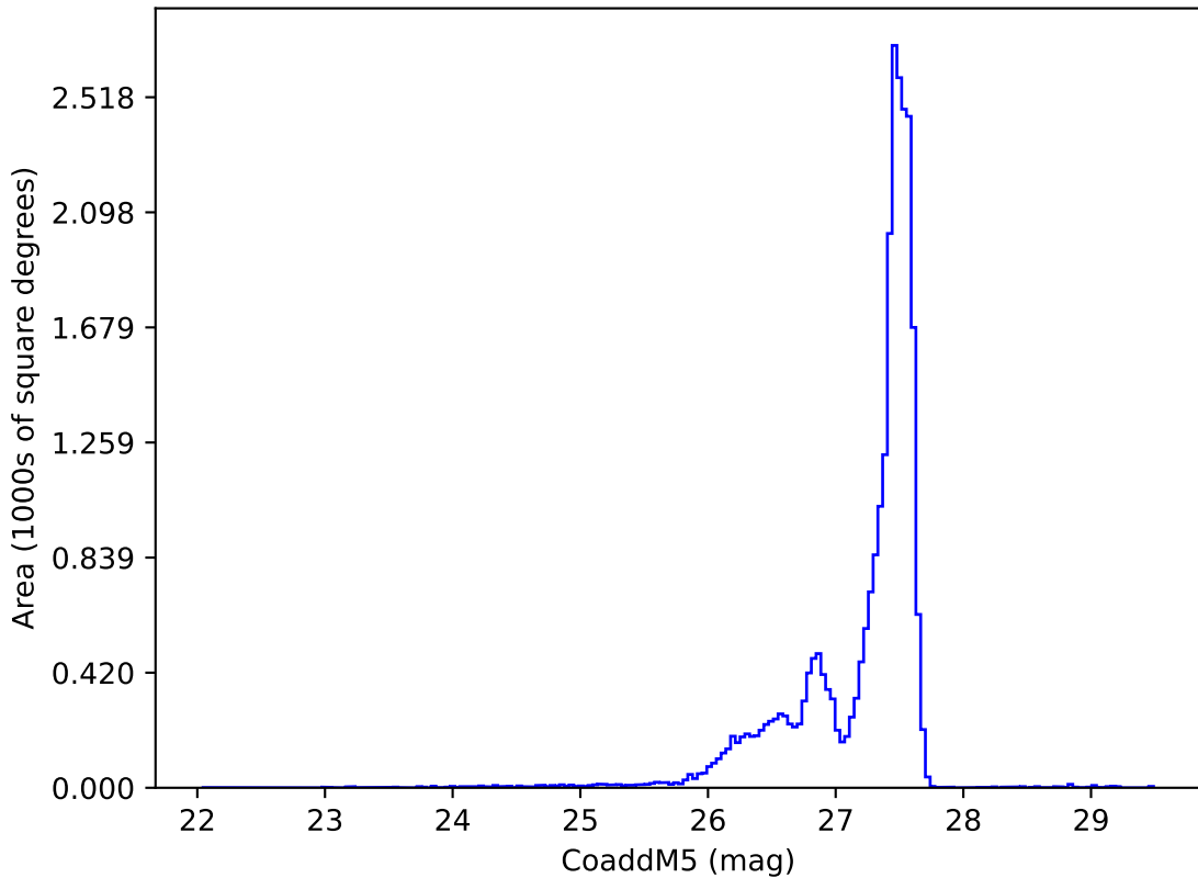
weather_cloudso12v3.4_10yrs : CoaddM5
