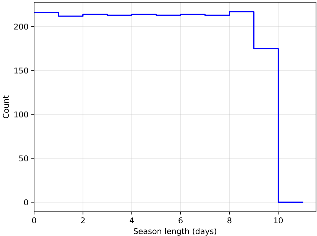
weather_cloudso12v3.4_10yrs DD:ECDFS all bands: SeasonLength
