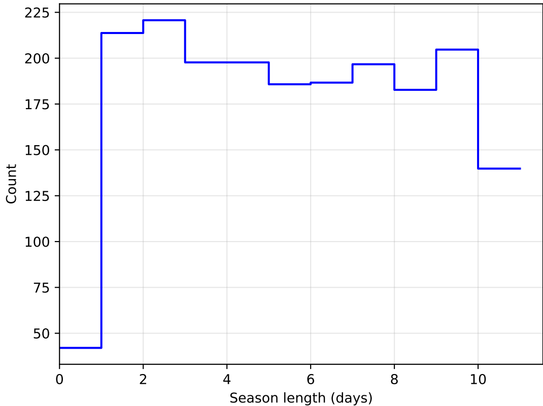
weather_cloudso12v3.4_10yrs DD: COSMOS all bands: SeasonLength
