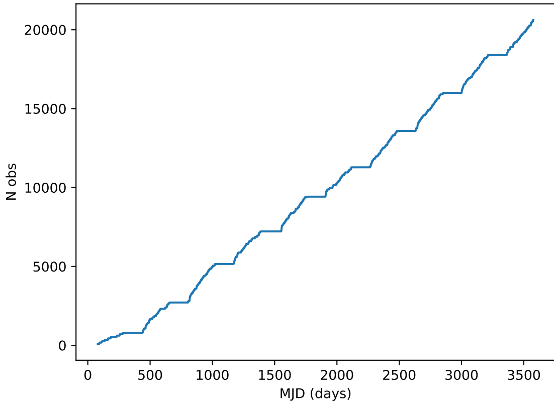
weather_cloudso12v3.4_10yrs all bands: DD:XMM_LSS Cumulative NVisits
