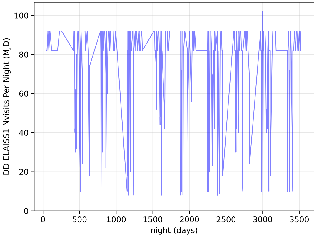
weather_cloudso12v3.4_10yrs all bands: DD:ELAISS1 Nvisits Per Night
