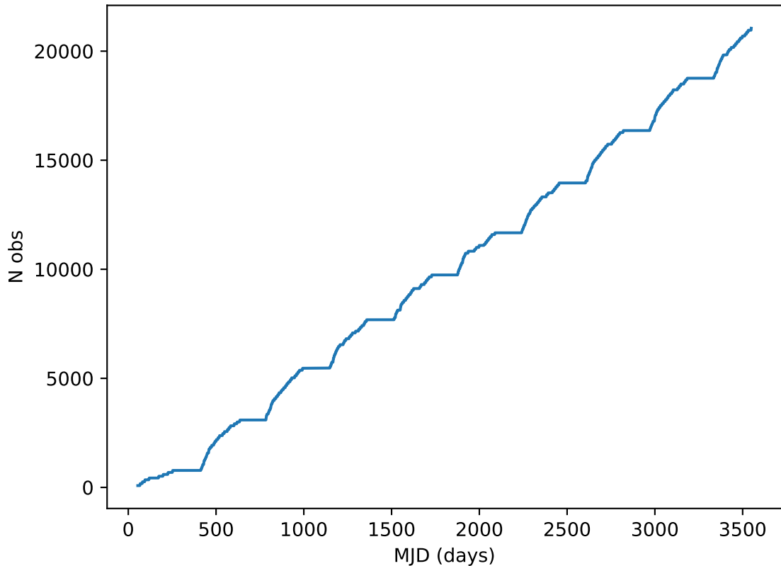
weather_cloudso12v3.4_10yrs all bands: DD:ELAISS1 Cumulative NVisits
