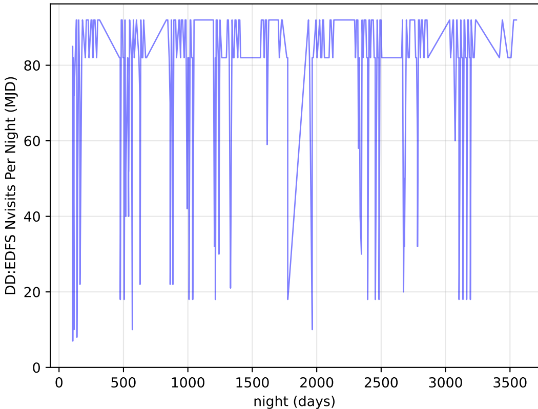
weather_cloudso12v3.4_10yrs all bands: DD:EDFS Nvisits Per Night
