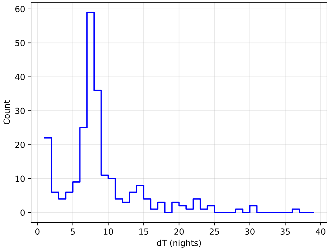
weather_cloudso12v3.4_10yrs all bands: DD:EDFS Delta Nights Histogram
