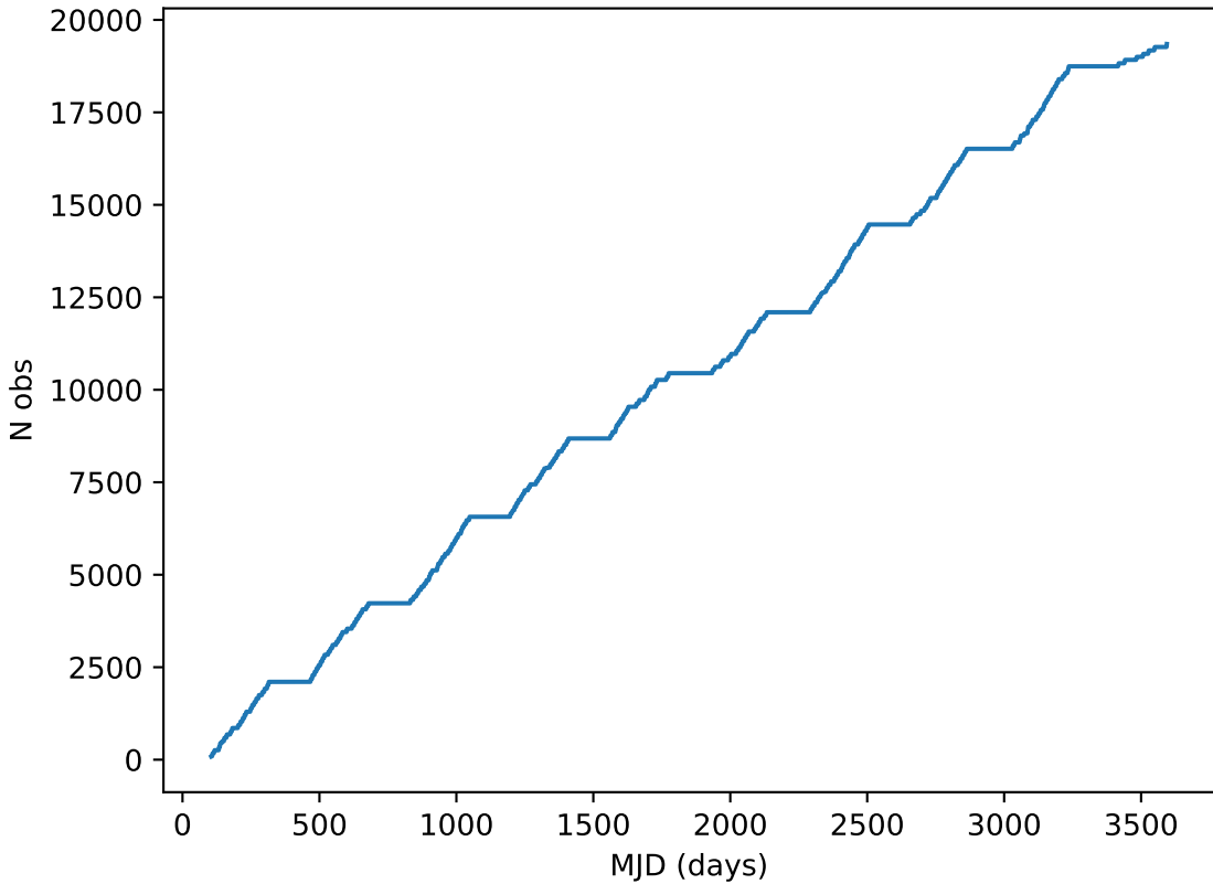
weather_cloudso12v3.4_10yrs all bands: DD:EDFS Cumulative NVisits
