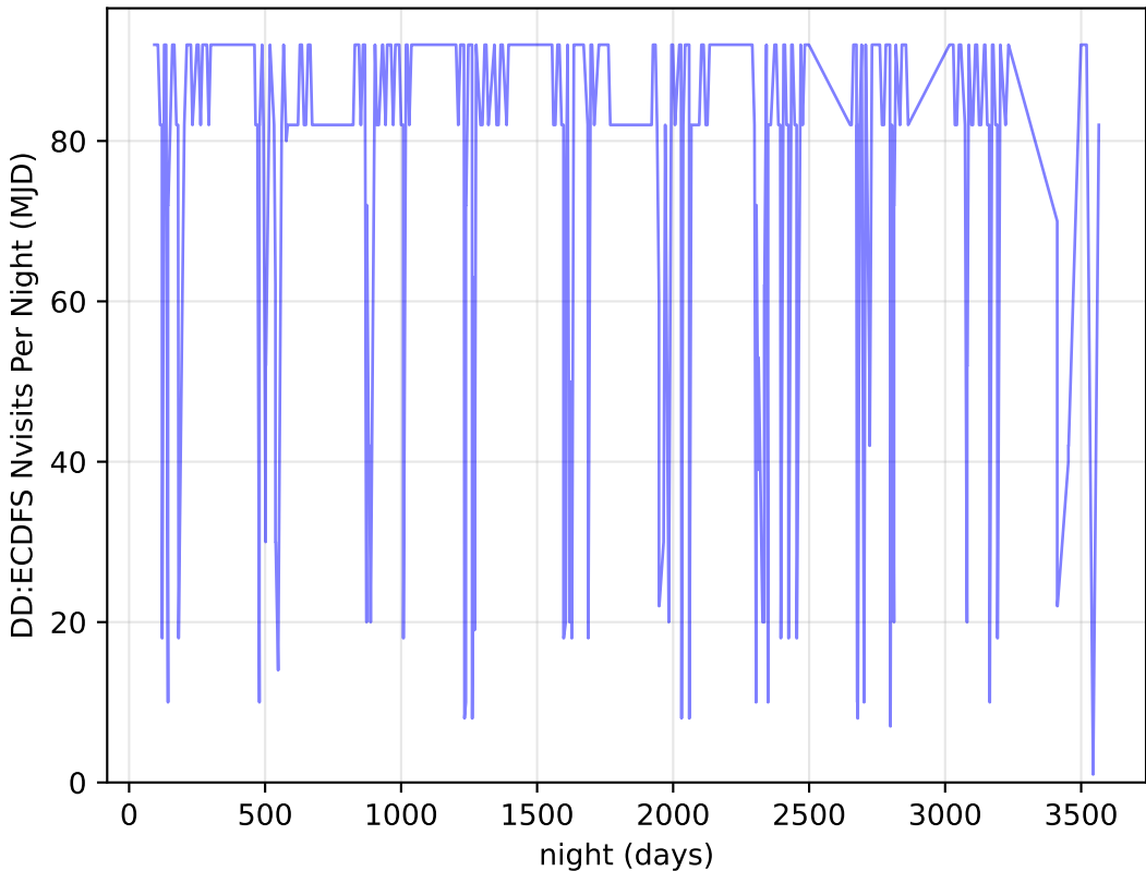
weather_cloudso12v3.4_10yrs all bands: DD:ECDFS Nvisits Per Night
