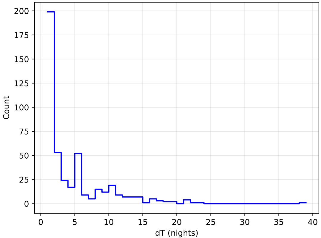
weather_cloudso12v3.4_10yrs all bands: DD: COSMOS Delta Nights Histogram
