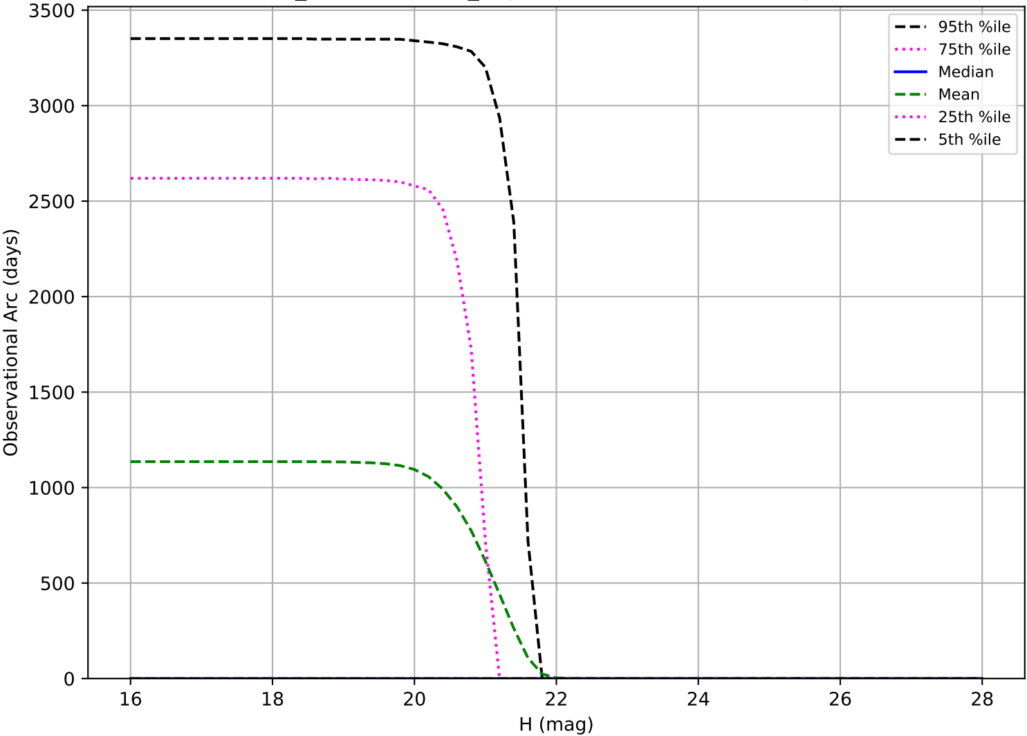
weather_cloudso10v3.4_10yrs: Observational Arc Length Vatra
