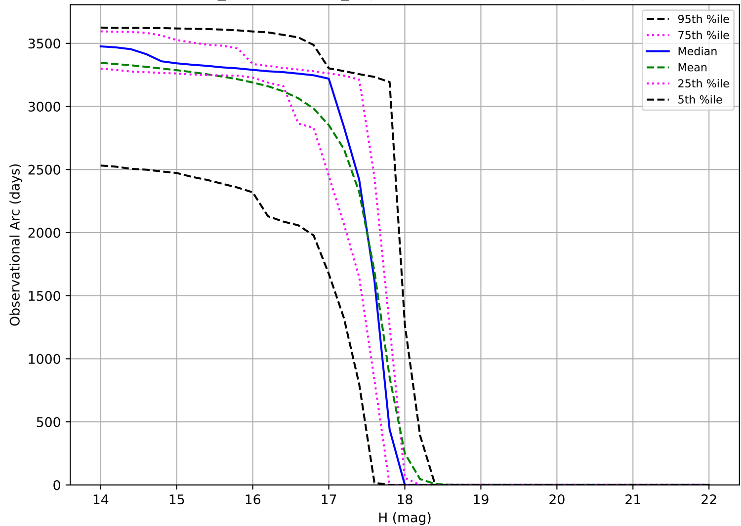
weather_cloudso10v3.4_10yrs: Observational Arc Length Trojan
