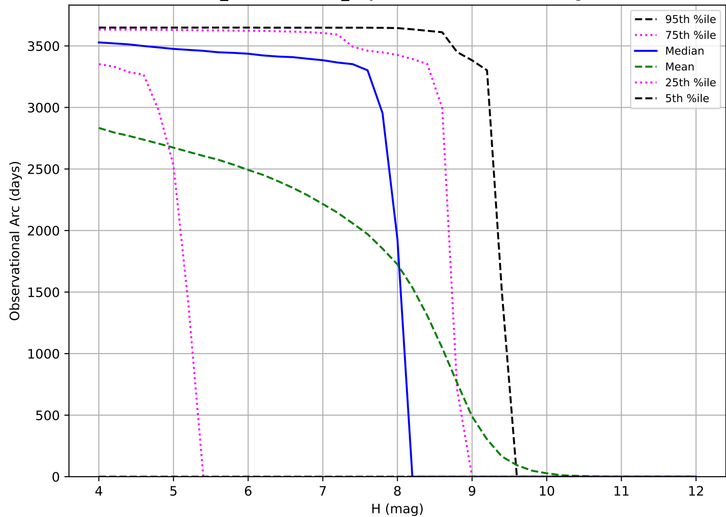
weather_cloudso10v3.4_10yrs: Observational Arc Length TNO
