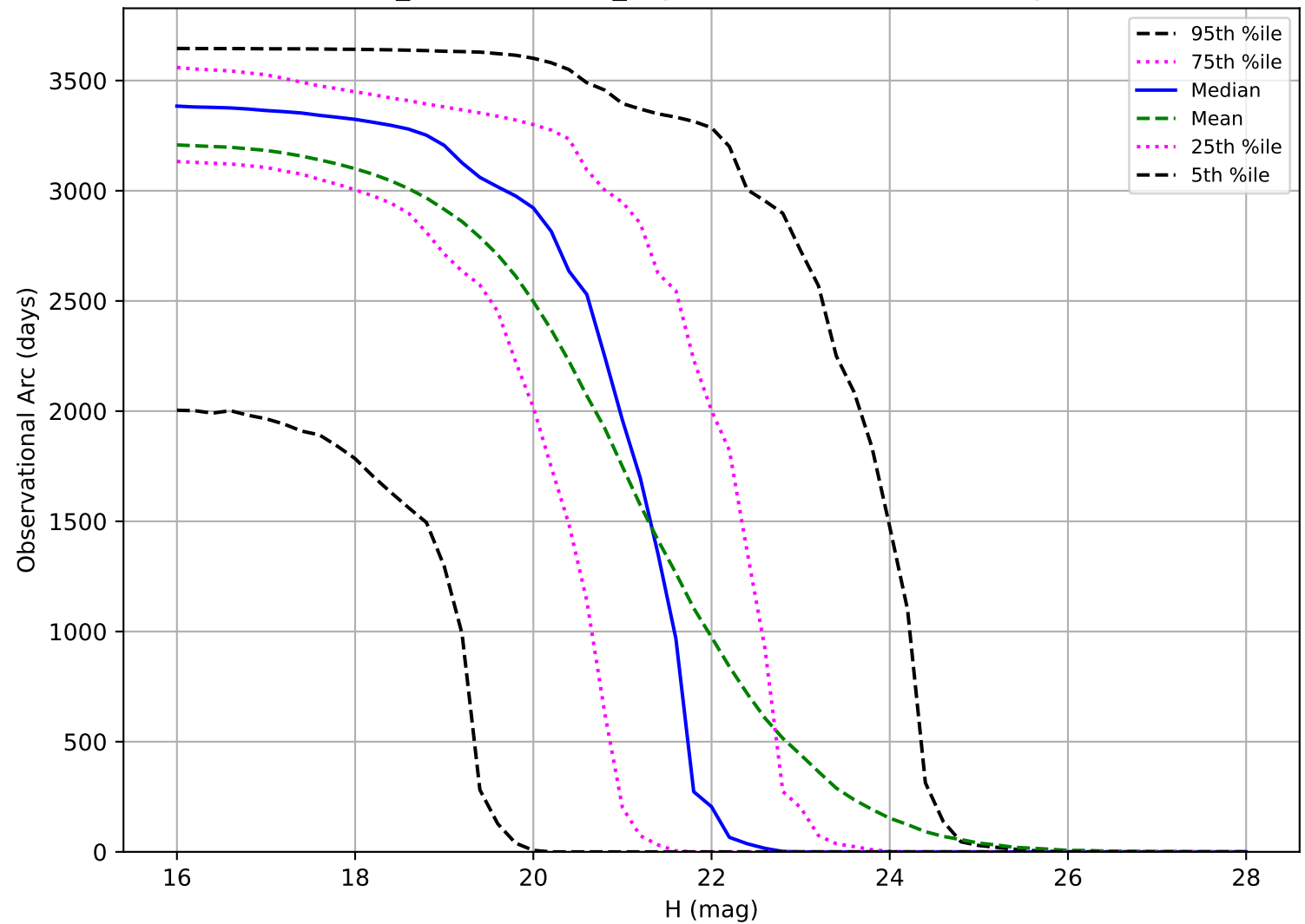
weather_cloudso10v3.4_10yrs: Observational Arc Length PHA
