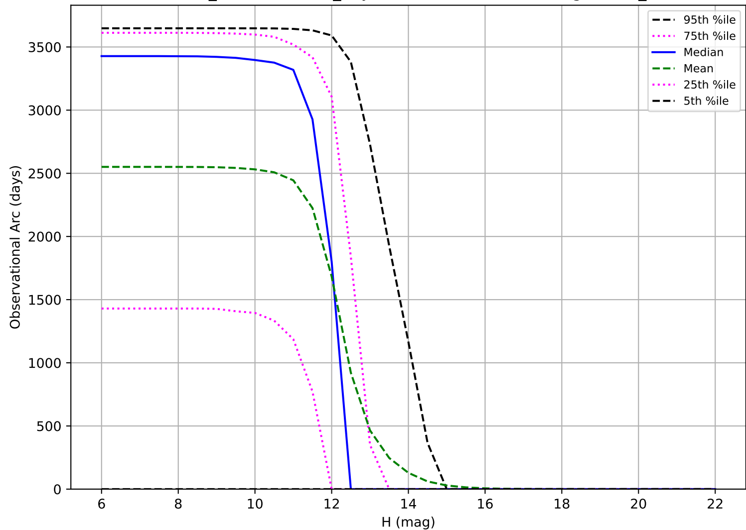
weather_cloudso10v3.4_10yrs: Observational Arc Length OCC_r20
