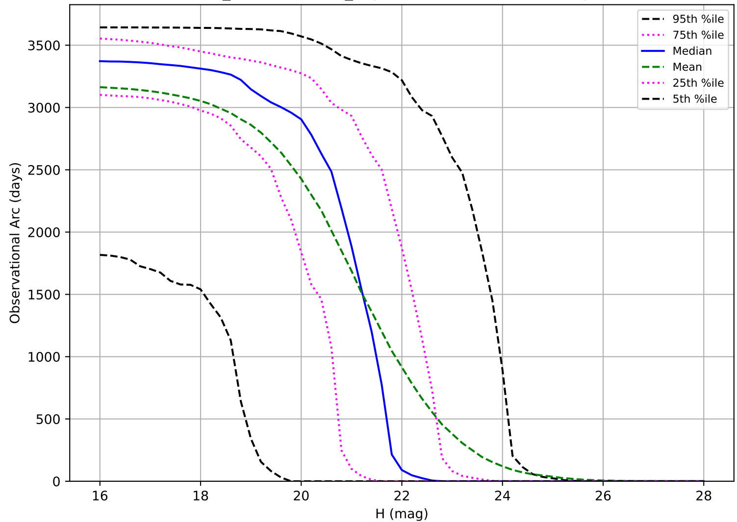
weather_cloudso10v3.4_10yrs: Observational Arc Length NEO
