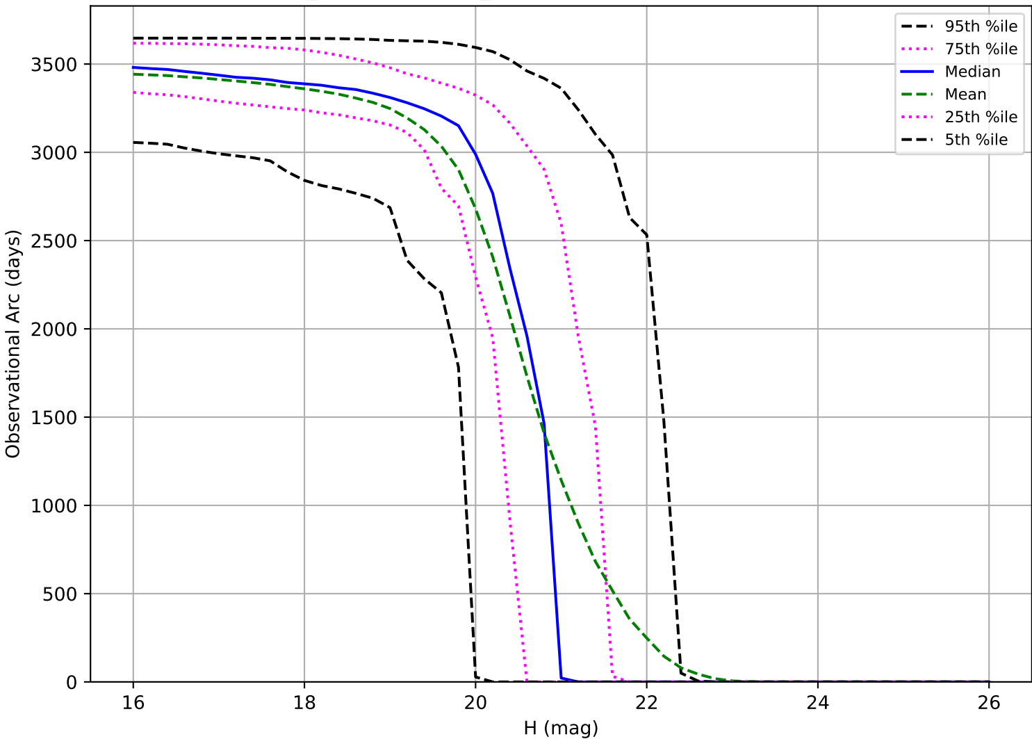
weather_cloudso10v3.4_10yrs: Observational Arc Length MBA
