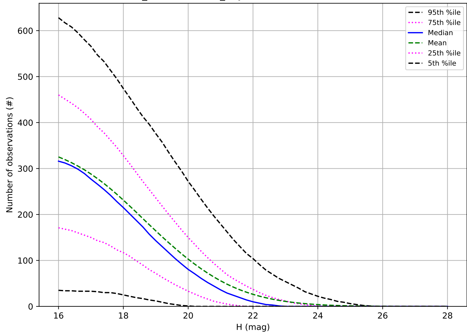
weather_cloudso10v3.4_10yrs: Number of observations NEO
