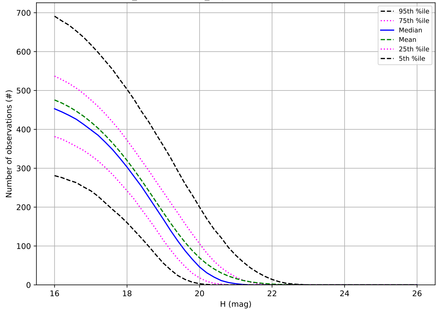
weather_cloudso10v3.4_10yrs: Number of observations MBA
