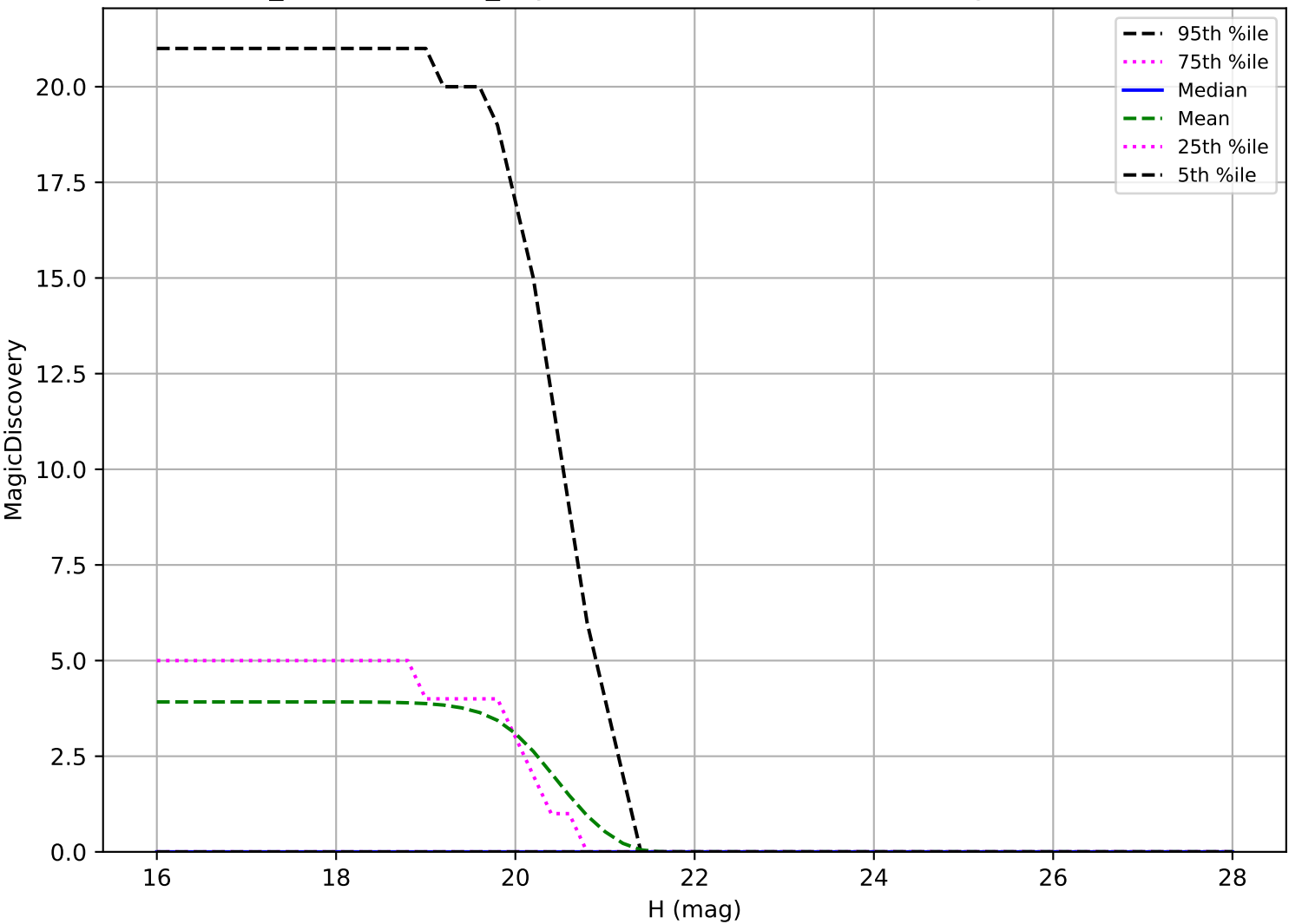
weather_cloudso10v3.4_10yrs: Vatira 6 detections in 60 nights detection loss
