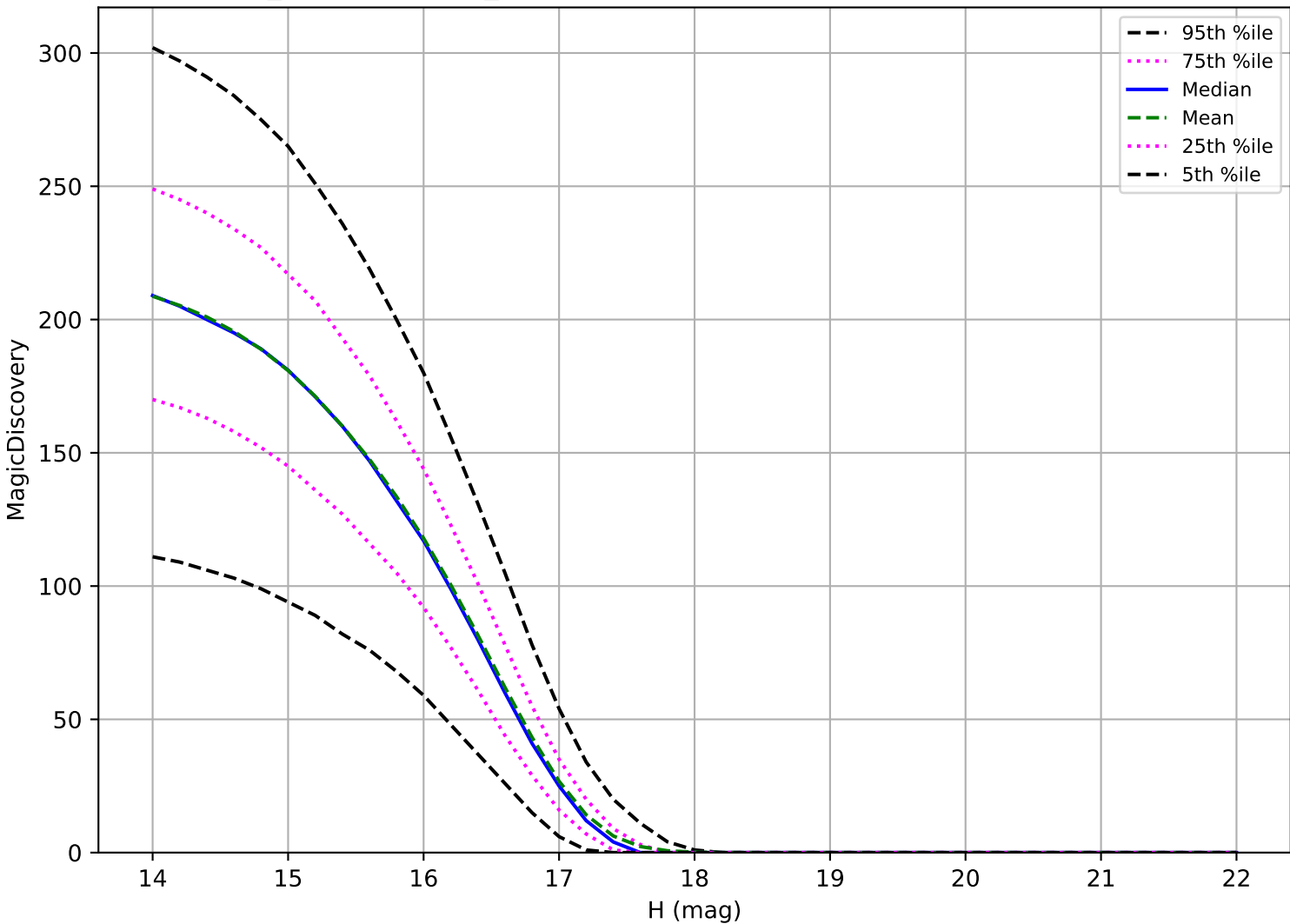
weather_cloudso10v3.4_10yrs: Trojan 6 detections in 60 nights detection loss
