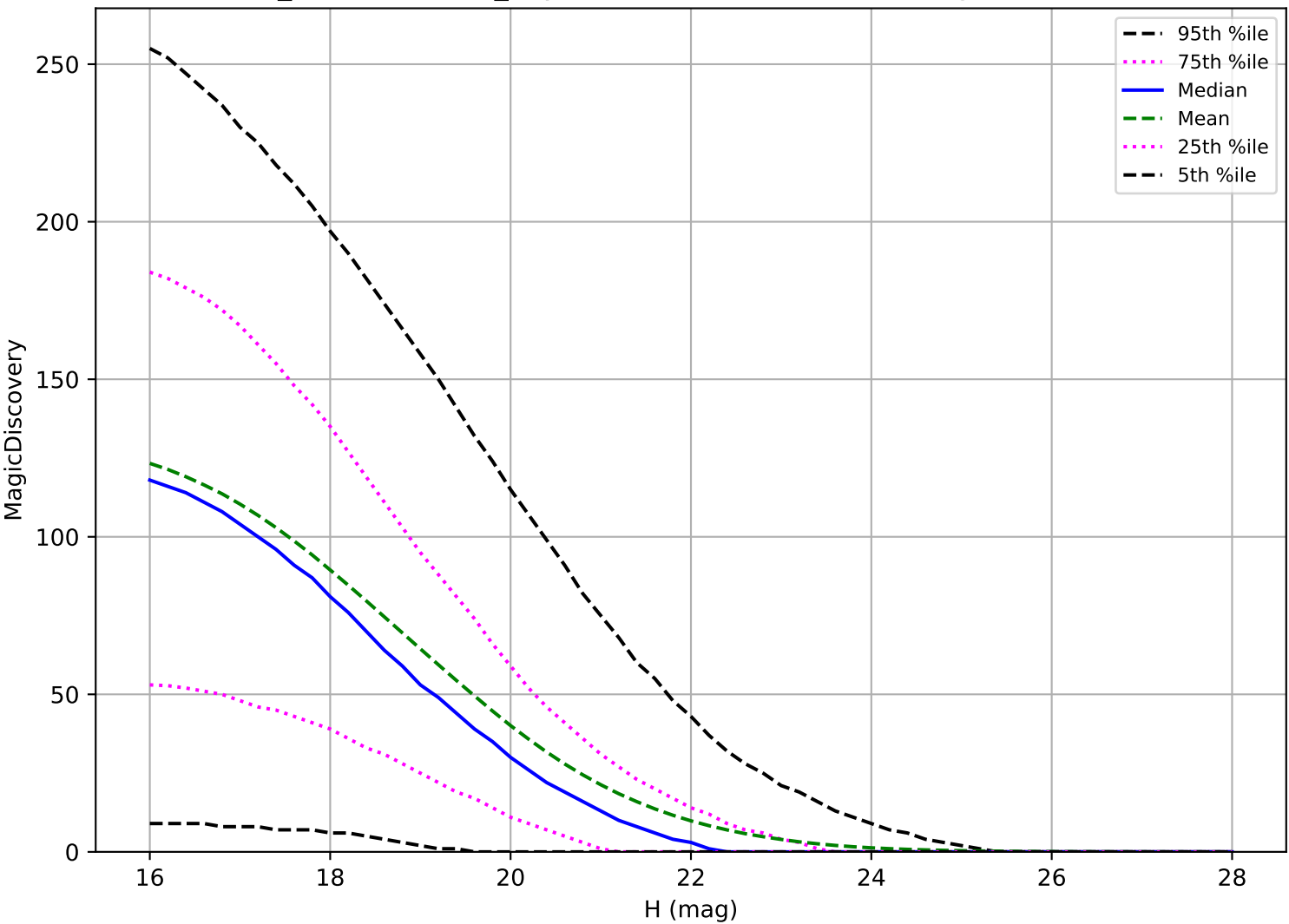
weather_cloudso10v3.4_10yrs: PHA 6 detections in 60 nights detection loss
