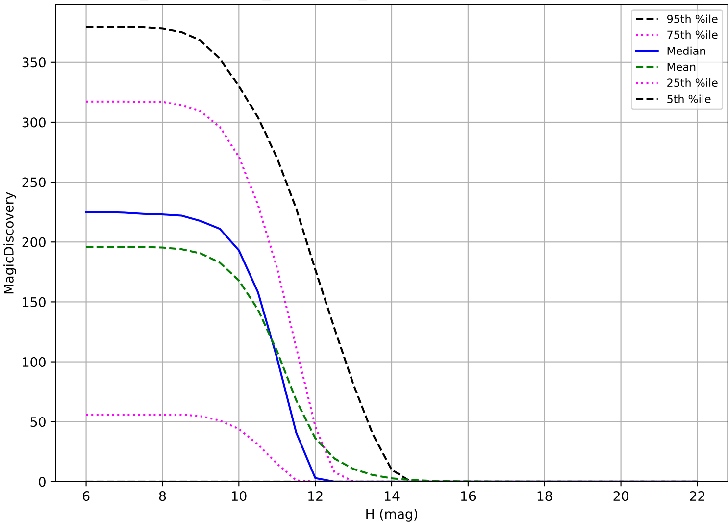
weather_cloudso10v3.4_10yrs: OCC_r20 6 detections in 60 nights detection loss
