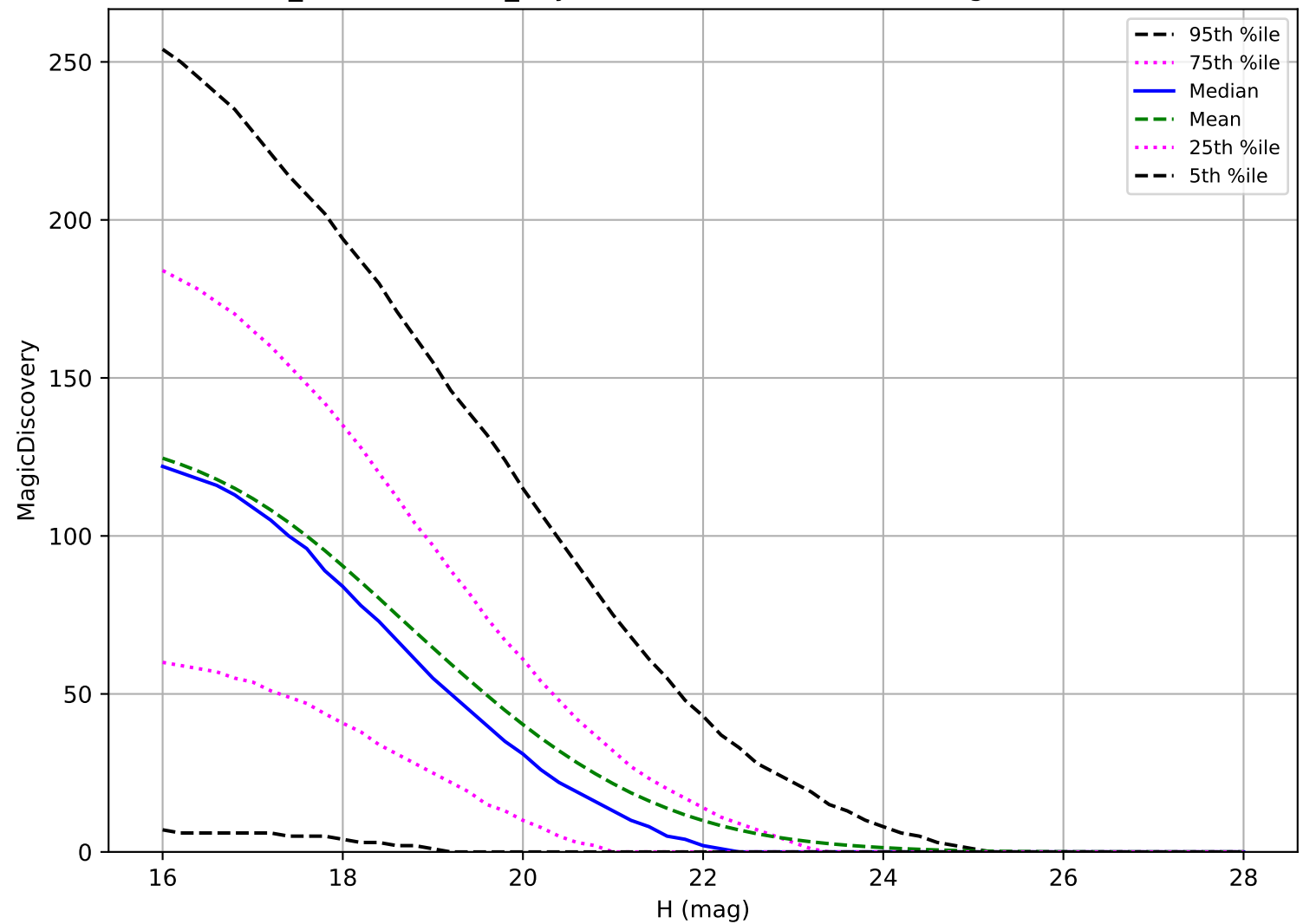
weather_cloudso10v3.4_10yrs: NEO 6 detections in 60 nights detection loss
