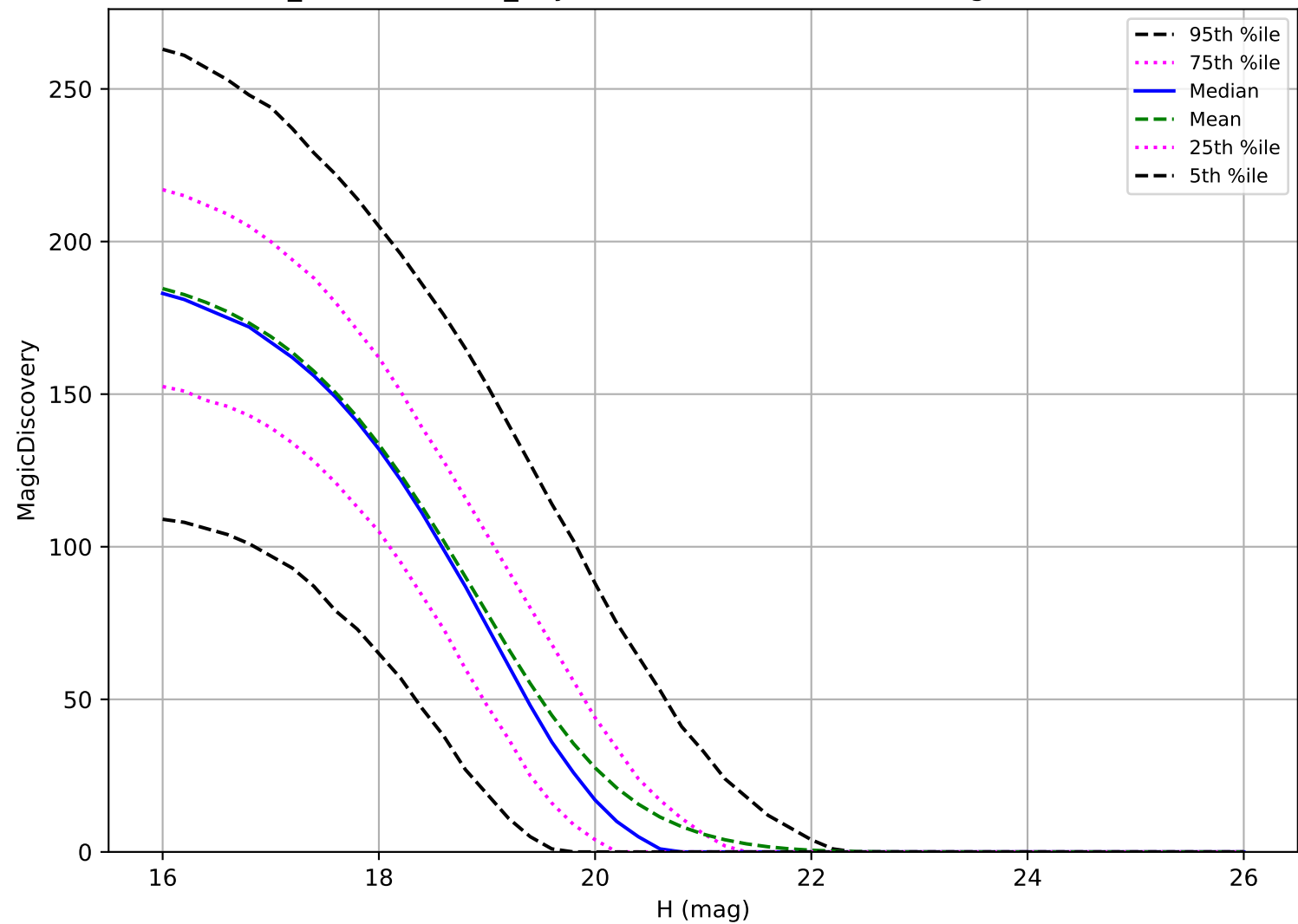
weather_cloudso10v3.4_10yrs: MBA 6 detections in 60 nights detection loss
