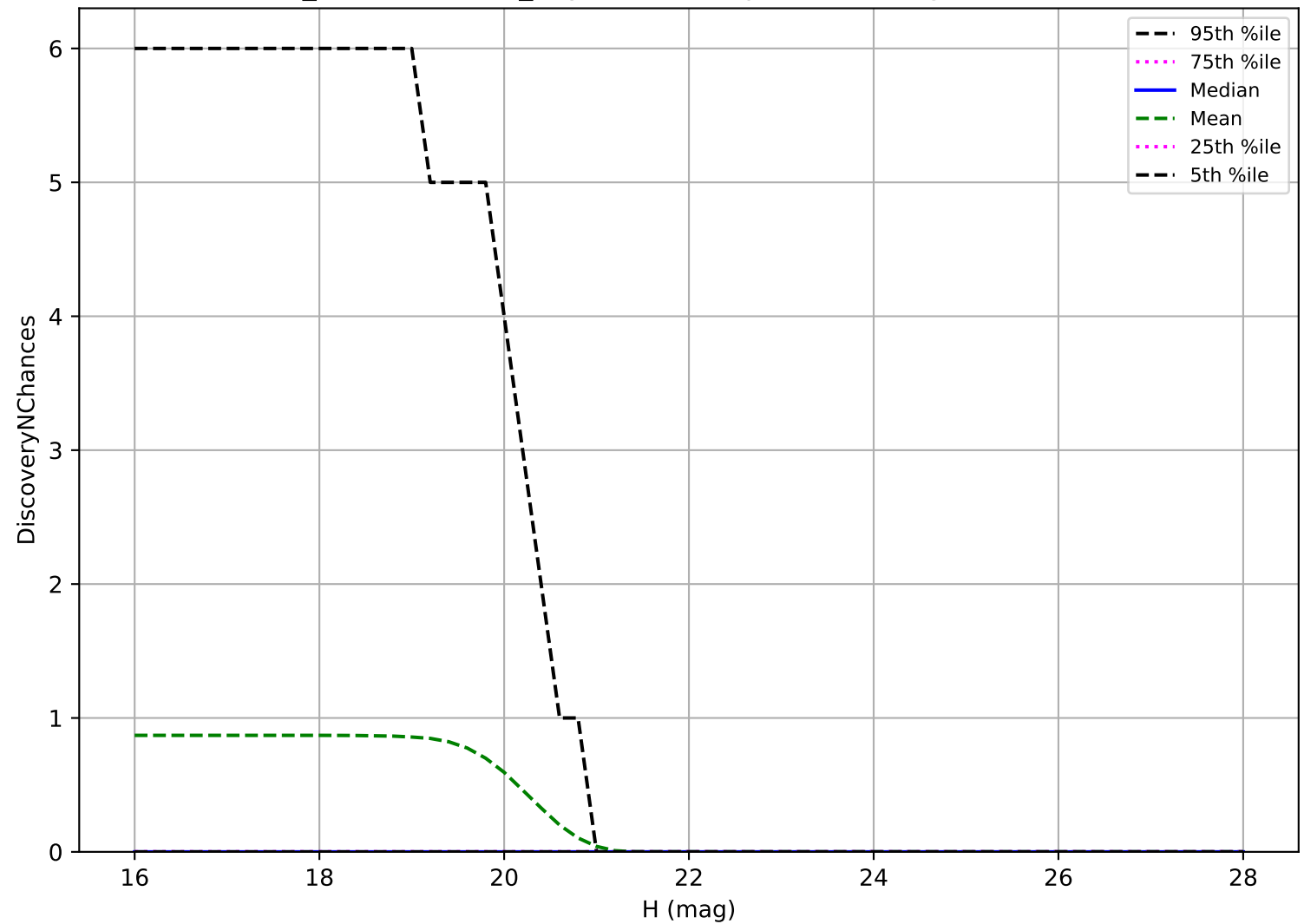
weather_cloudso10v3.4_10yrs: Vatira 3 pairs in 15 nights detection loss
