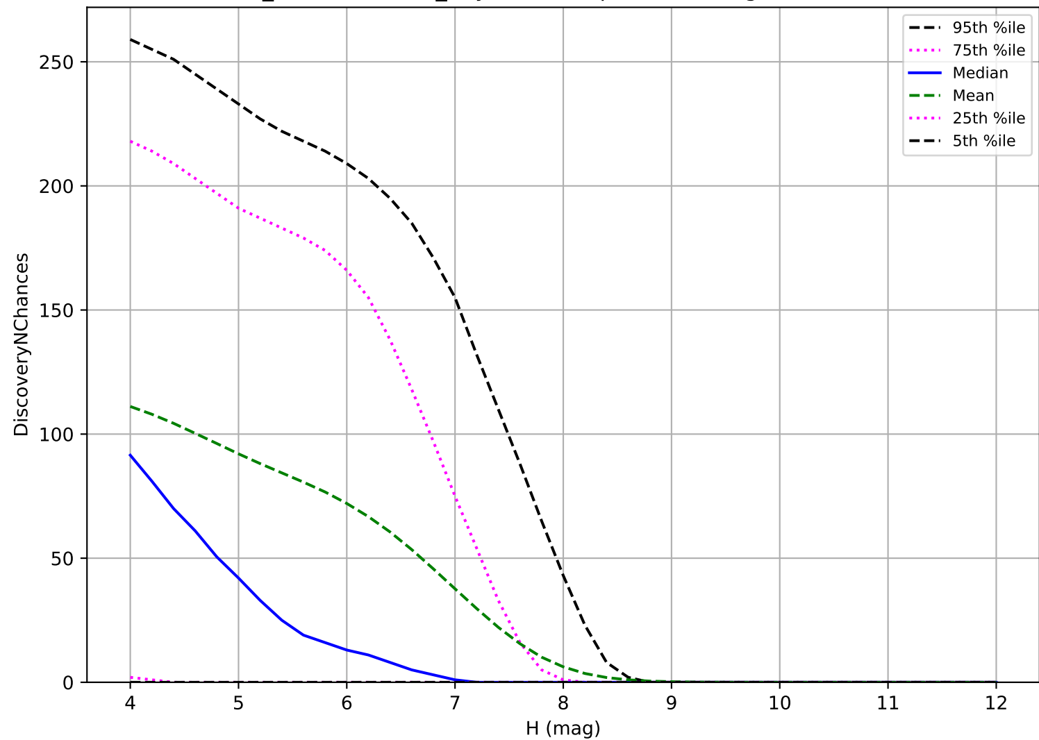
weather_cloudso10v3.4_10yrs: TNO 3 pairs in 15 nights detection loss
