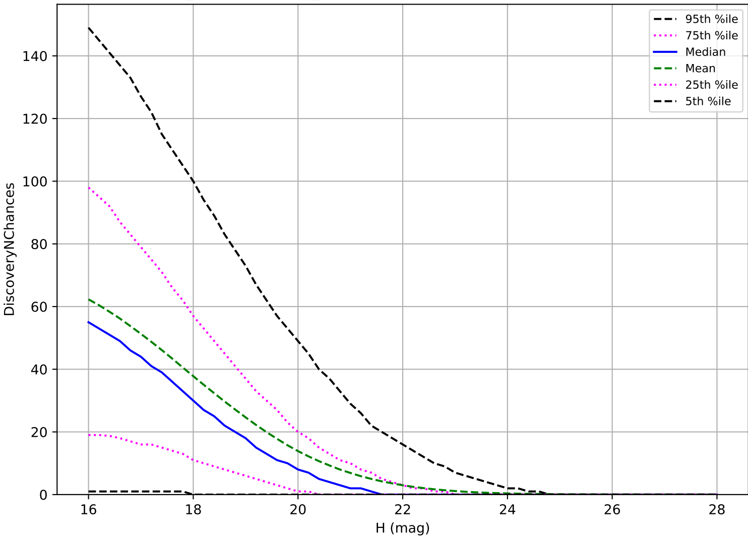
weather_cloudso10v3.4_10yrs: PHA 3 pairs in 15 nights detection loss
